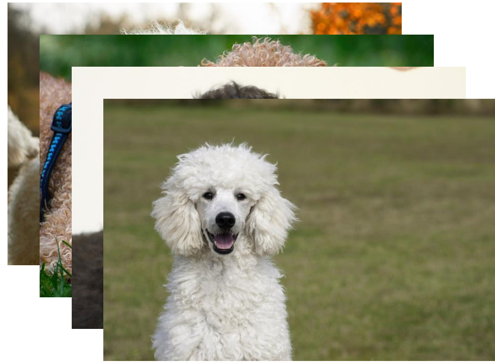
Training Data
