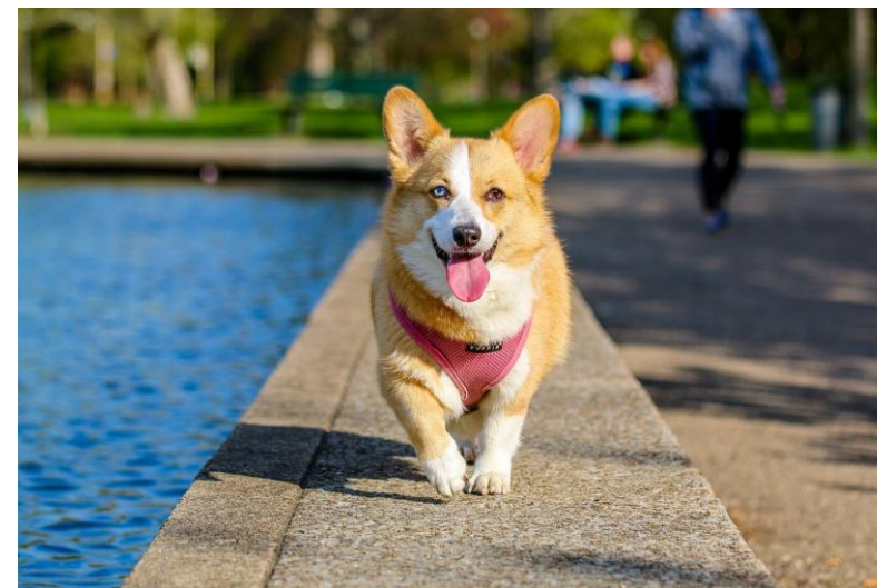
Test Data
