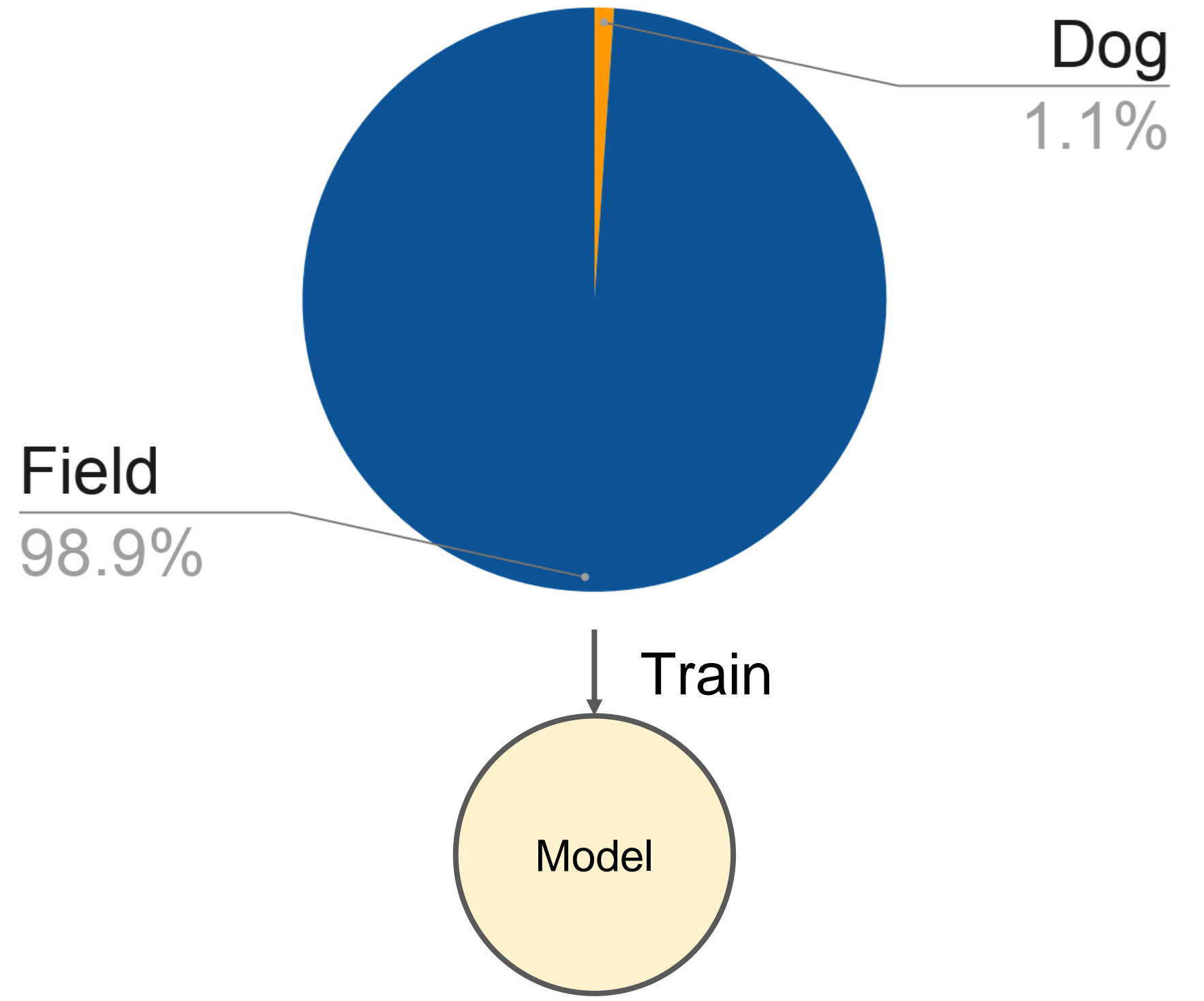
Dataset Classes
